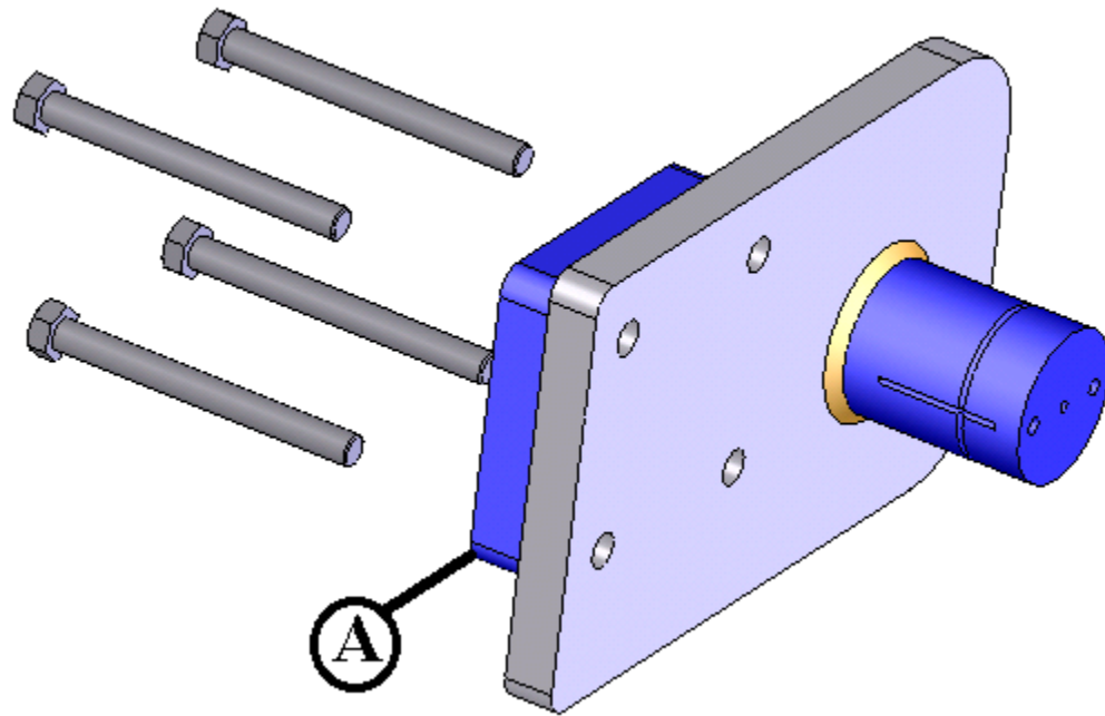
Figure 2 – Spacer Plate Installation (LH Side Shown)
